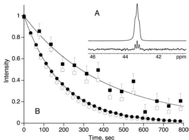
Figure 2. (A) Proton-coupled ^{15}\text{N} spectra of hyperpolarized solutions of ^{15}\text{N} -enriched choline (top; 10° pulse), and of choline- d_9 (bottom; 15° pulse). (B) Decays of ^{15}\text{N} hyperpolarization in ^{15}\text{N} -choline (○) and choline- d_9 (□), obtained using a series of 10° and 15° pulses, respectively. The curves represent three-parameter exponential fits to signal amplitudes that were corrected for magnetization losses due to the small-angle pulses (filled symbols).
