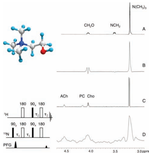
Figure 1. (A) Conventional ^1\text{H} NMR of ^{15}\text{N} -enriched choline in \text{H}_2\text{O} . (B) ^1\text{H} DNP-NMR of ^{15}\text{N} -choline, using inverse-INEPT. (C) ^{15}\text{N} -filtered ^1\text{H} spectrum of a mixture of 0.3 M natural-abundance acetylcholine (ACh) and phosphocholine (PC) and 1.3 mM ^{15}\text{N} -choline (Cho), 256 scans. (D) The inverse-INEPT ^1\text{H} DNP-NMR spectrum of a mixture of natural-abundance Cho and ACh. Left: Molecular structure of choline and inverse-INEPT pulse sequence. Proton signals that do not originate from ^{15}\text{N} magnetization were suppressed by two pulsed field gradients (PFG) in a 10:1 ratio.
